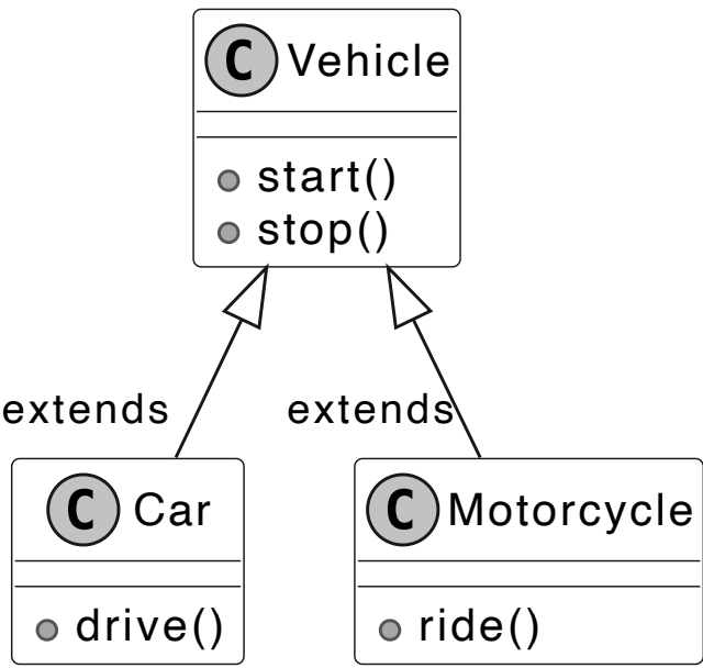
Hierarchical inheritance
