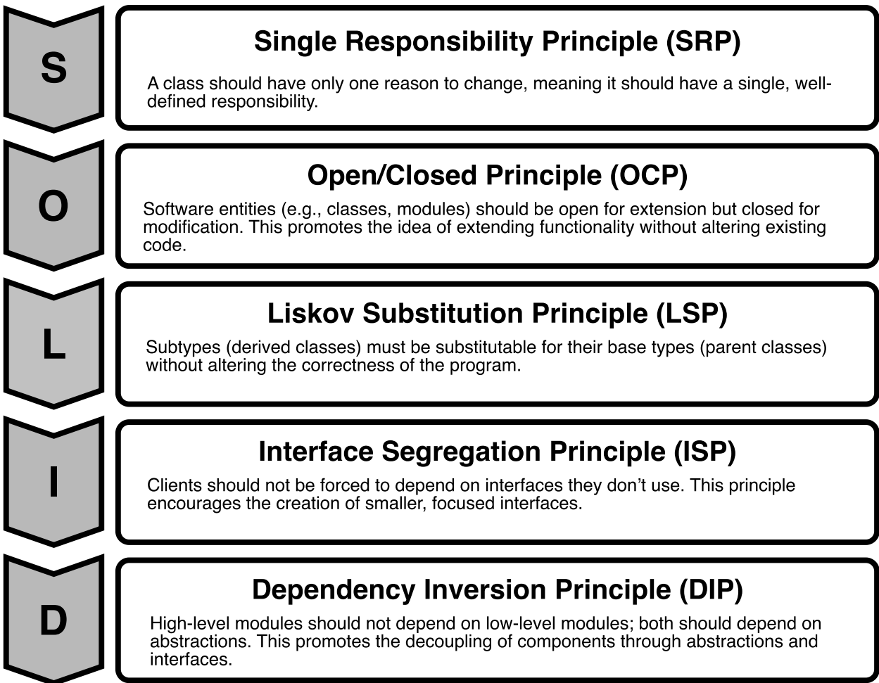
SOLID Principles
